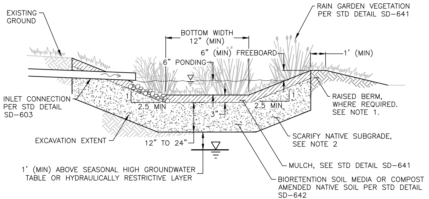
SECTION A NTS SD-601
